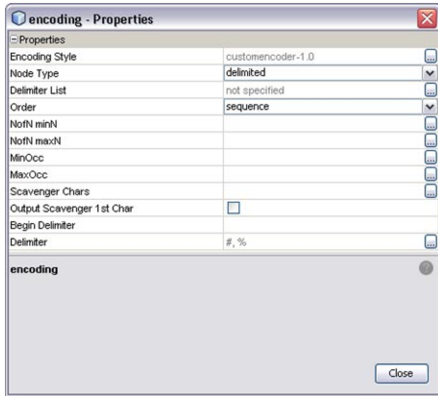
FIGURE 19 Field_1 Properties
