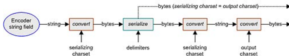
FIGURE 26 encodeToBytes()
