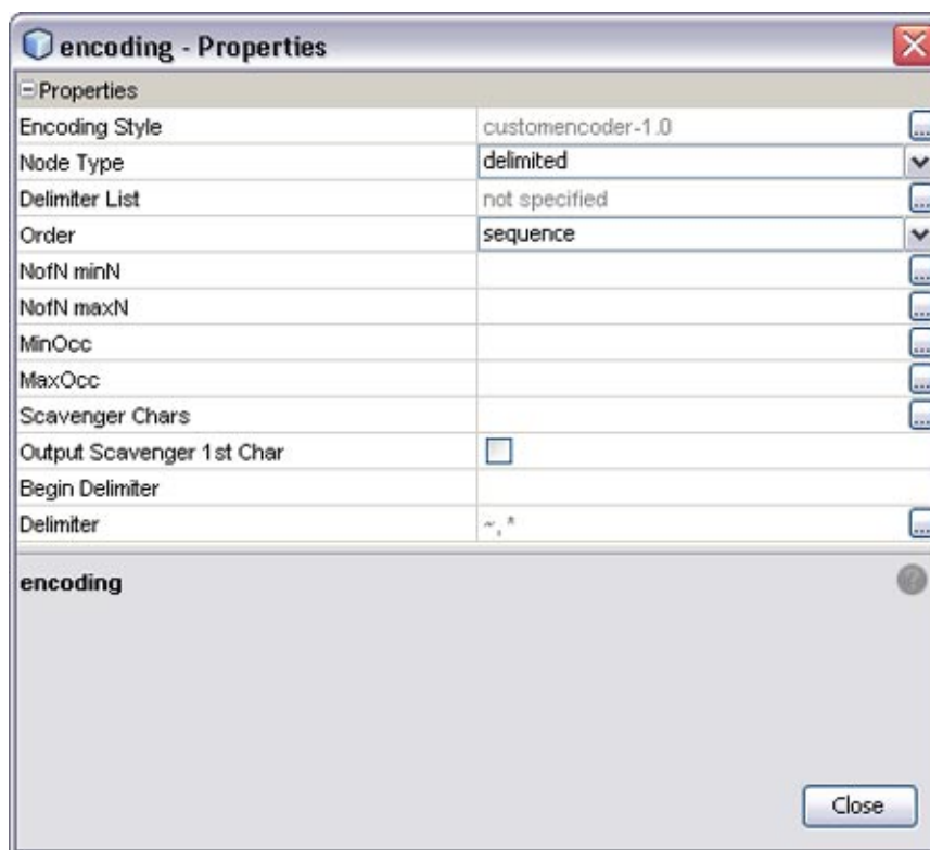
FIGURE 18 Element_2 Properties
