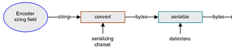
FIGURE 24 Encoding Process
